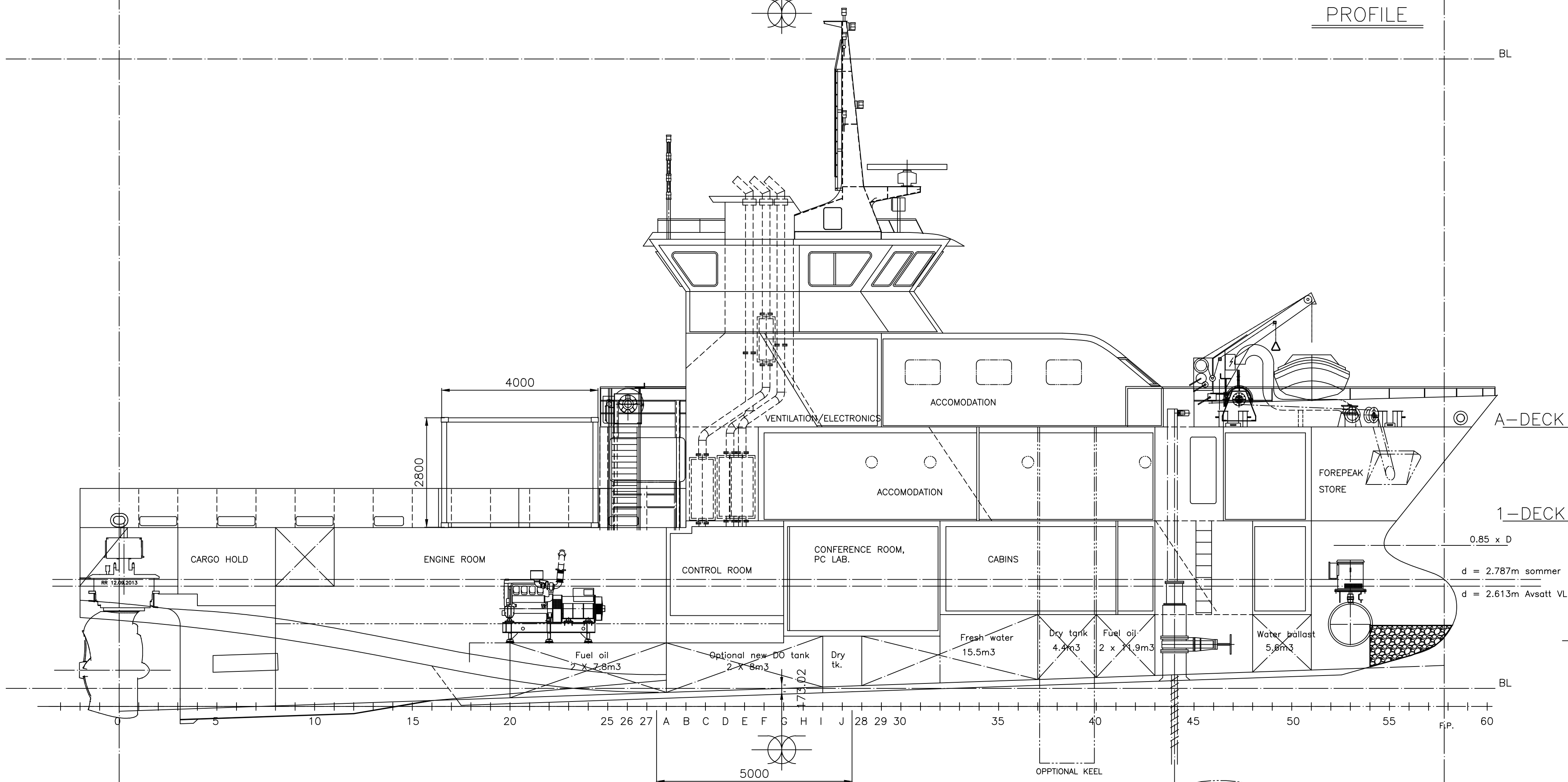
PROFILE
