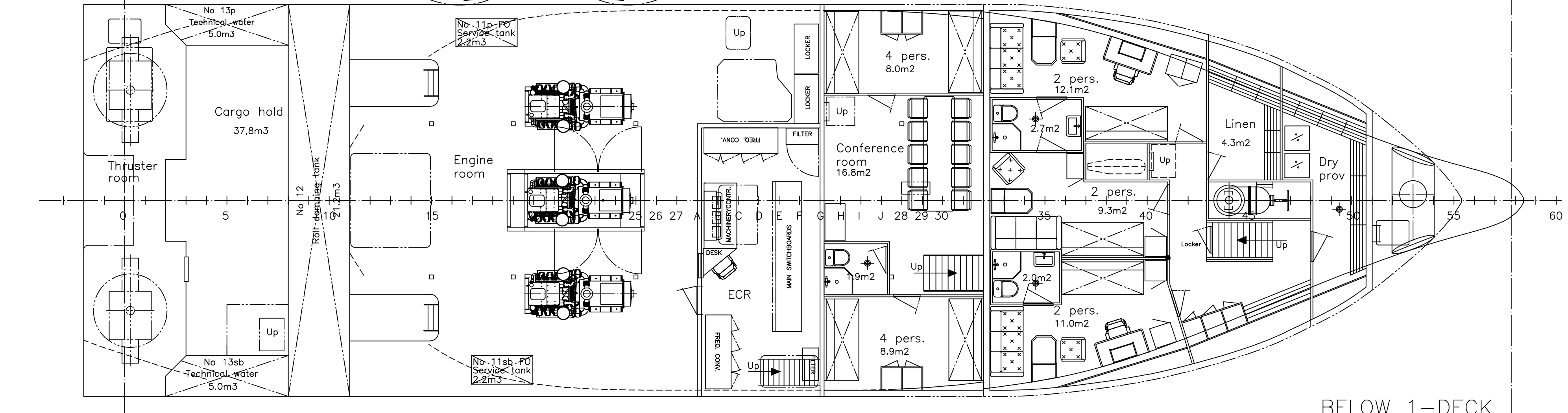
BELOW 1-DECK
