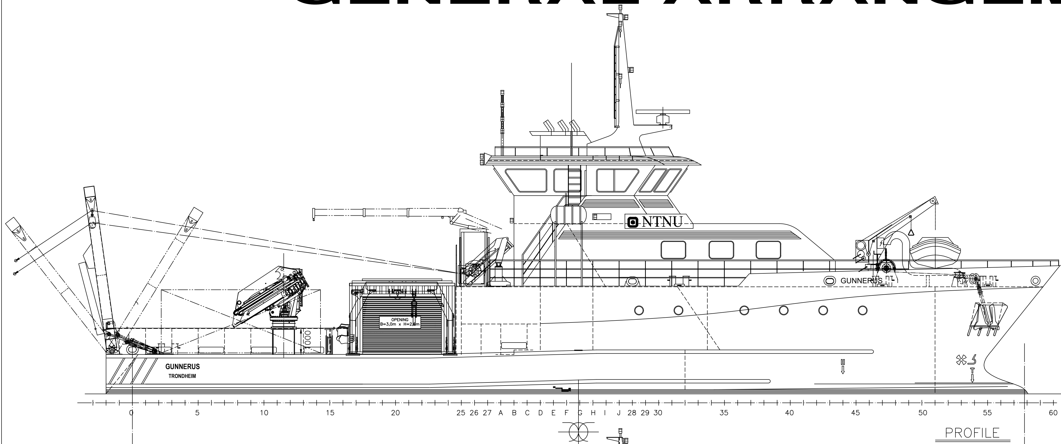
PROFILE
