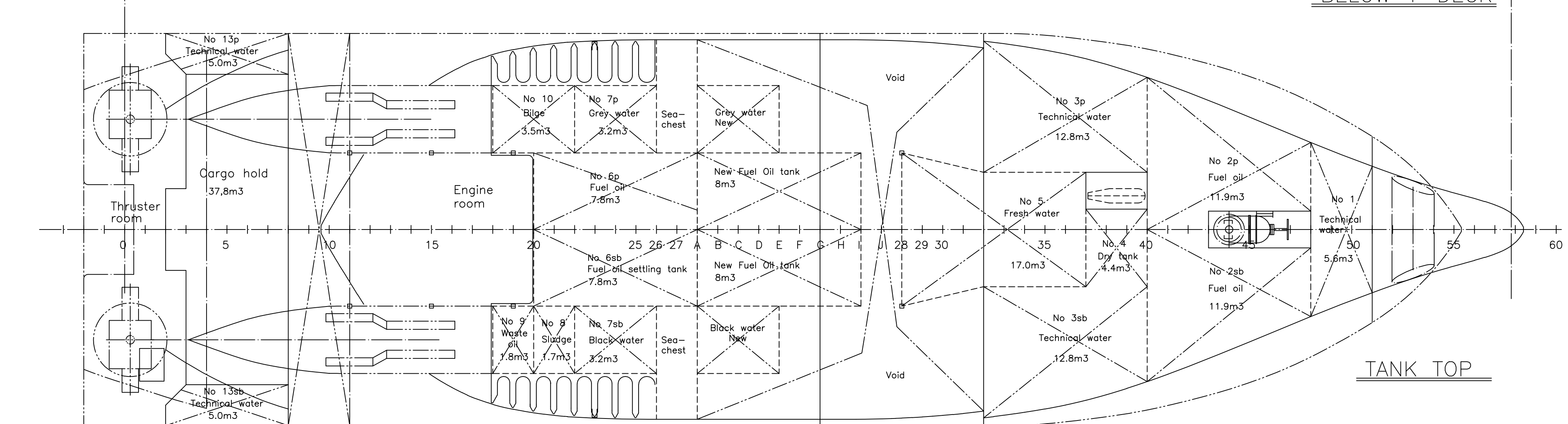
BELOW 1-DECK
