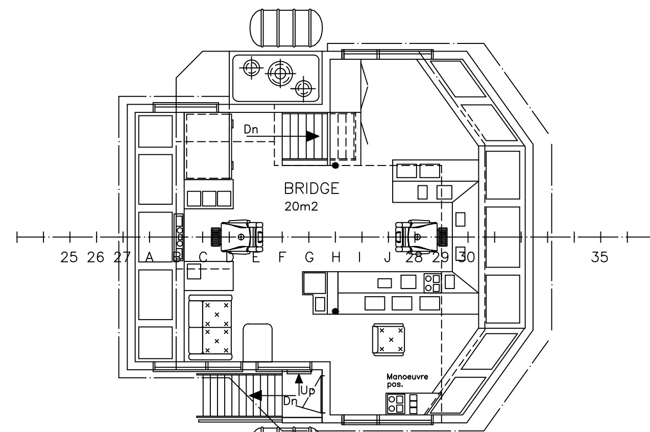
WHEEL HOUSE
